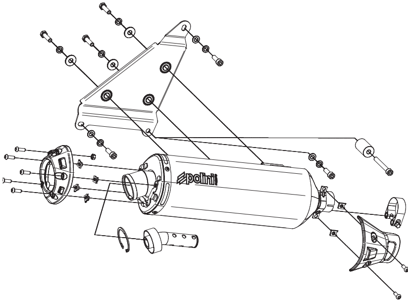
Silencer
